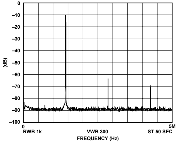
Figure 19. f_{MCLK} = 10 \text{ MHz} ; f_{OUT} = 1.43 \text{ MHz} = f_{MCLK}/7 , Frequency Word = 2492492
