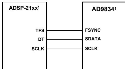
Figure 34. ADSP-21xx to AD9834 Interface
