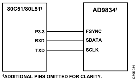
Figure 36. 80C51/80L51 to AD9834 Interface
