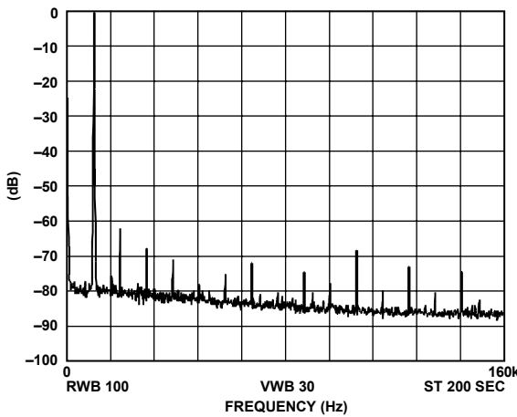
Figure 21. f_{MCLK} = 50 \text{ MHz} ; f_{OUT} = 12 \text{ kHz} , Frequency Word = 000FBA9
