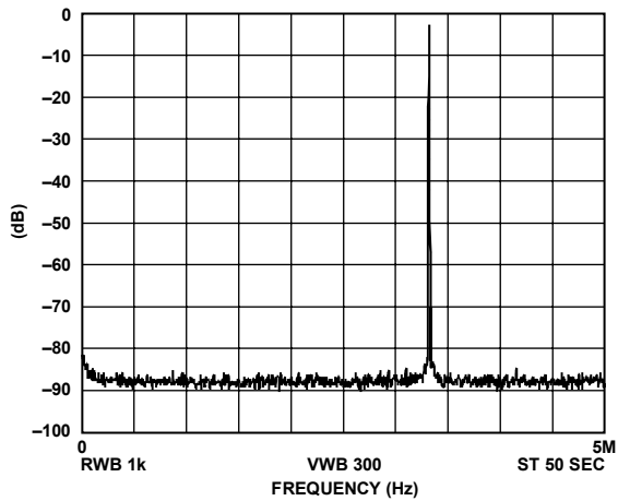
Figure 20. f_{MCLK} = 10 \text{ MHz} ; f_{OUT} = 3.33 \text{ MHz} = f_{MCLK}/3 , Frequency Word = 5555555
