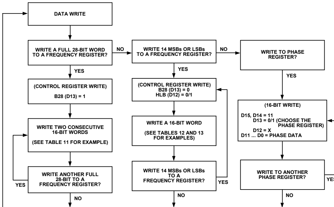
Figure 32. Data Write
