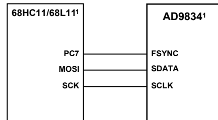
Figure 35. 68HC11/68L11 to AD9834 Interface
