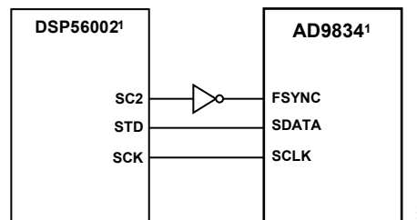
Figure 37. DSP56002 to AD9834 Interface
